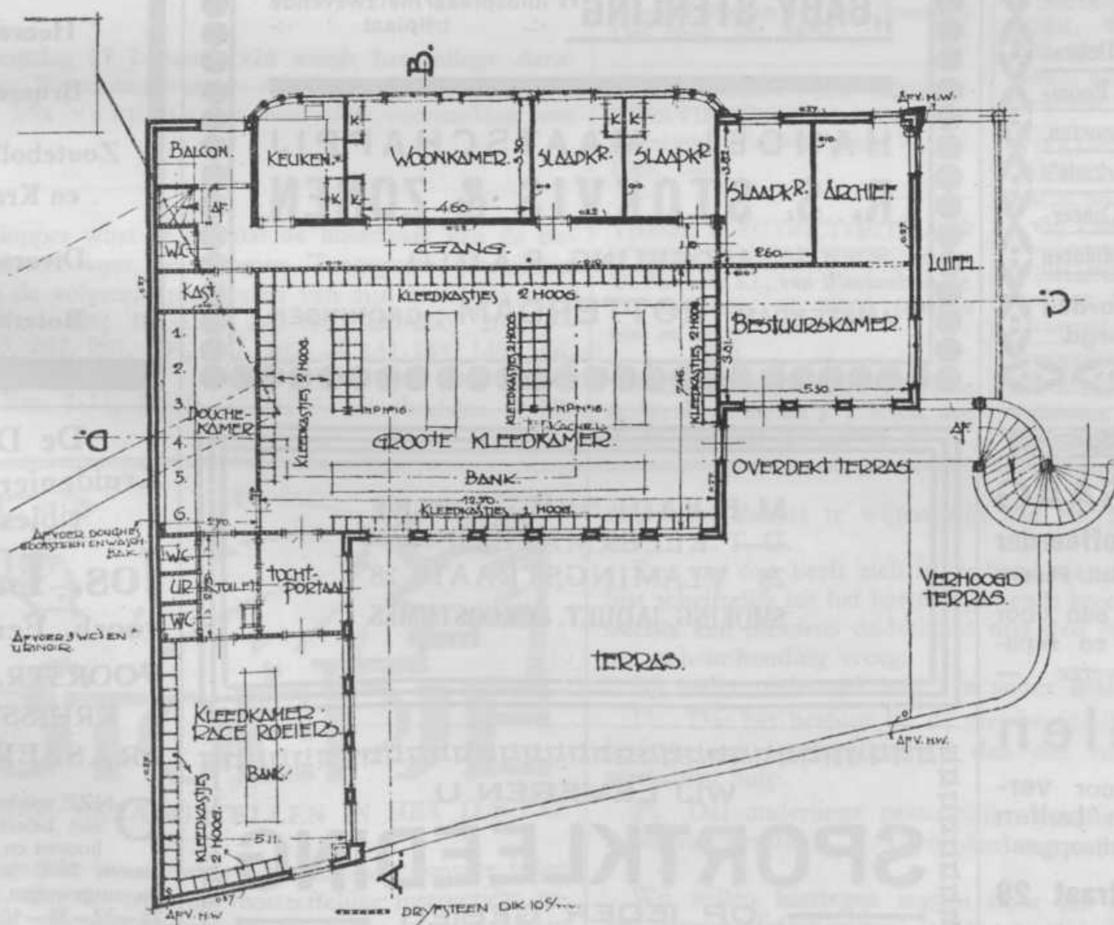
PLAN VERDIEPING.
