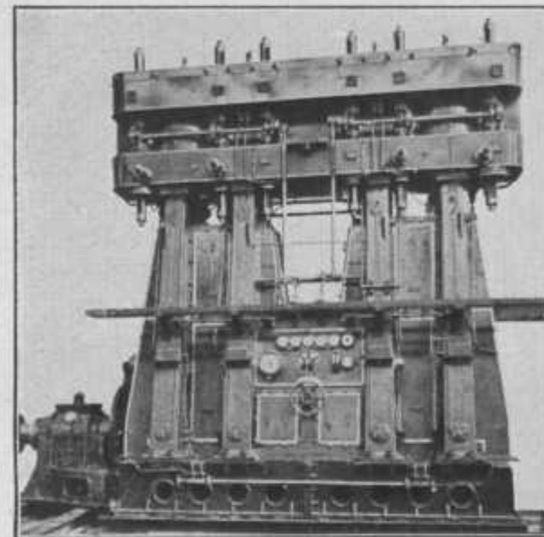
SCHEEPSMACHINES
