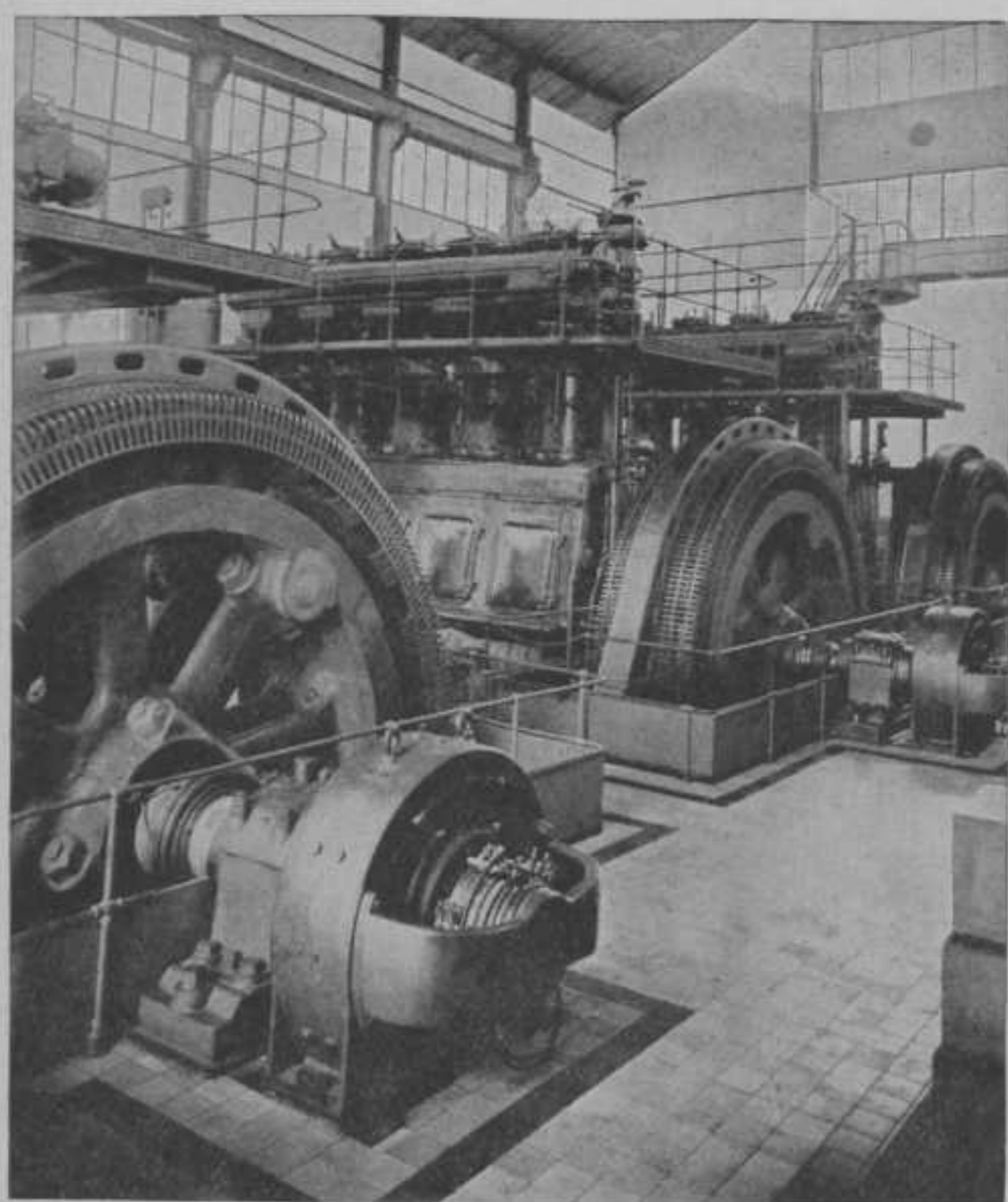
ELECTRISCHE CENTRALE WILLEMSTAD (CURAÇAO)
