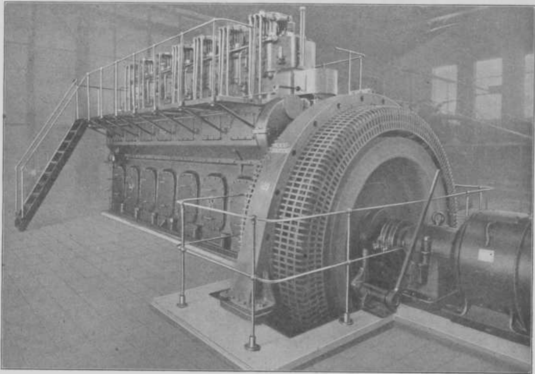
7-CYLINDER WERKSPOOR COMPRESSORLOOZE DIESELMOTOR 785 P.K. TYPE T.M. 397
