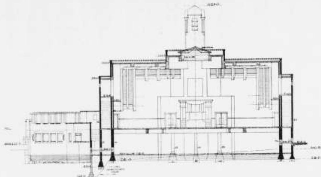
"FIRST CHURCH OF CHRIST SCIENTIST"
