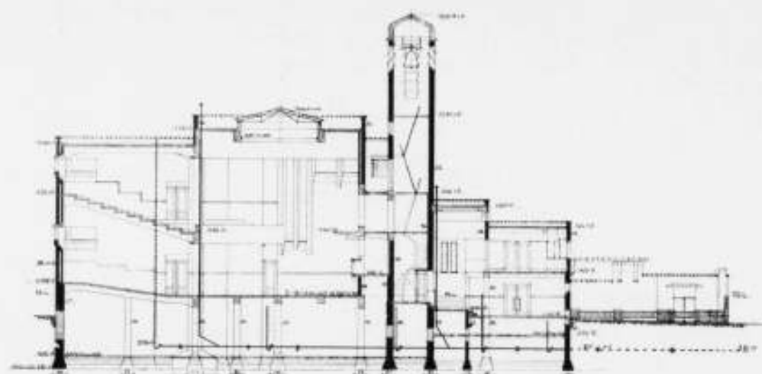
"FIRST CHURCH OF CHRIST SCIENTIST"
