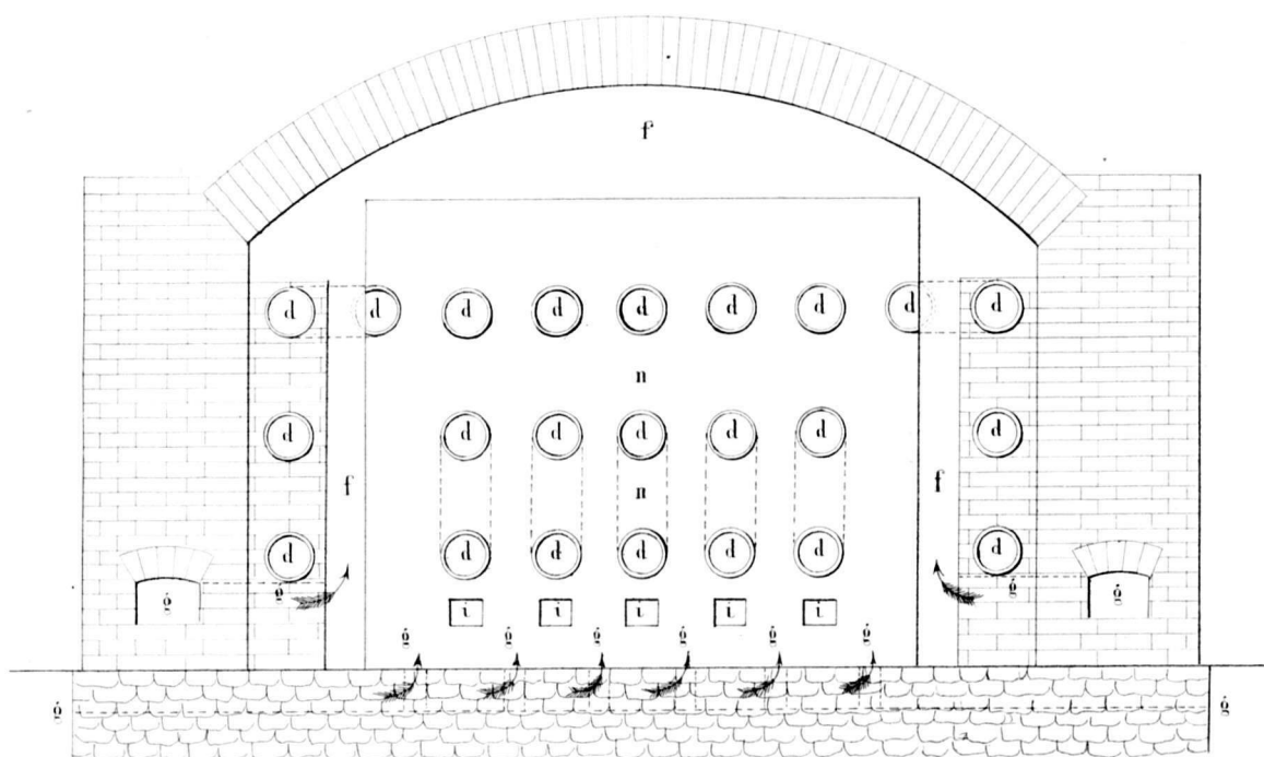
Doorsnede over EF.
