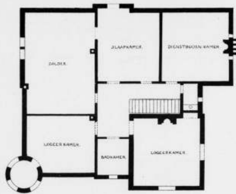
ZOLDERVERDIEPING.
