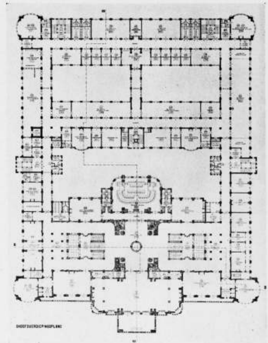
HOOFVERDIEPING.
