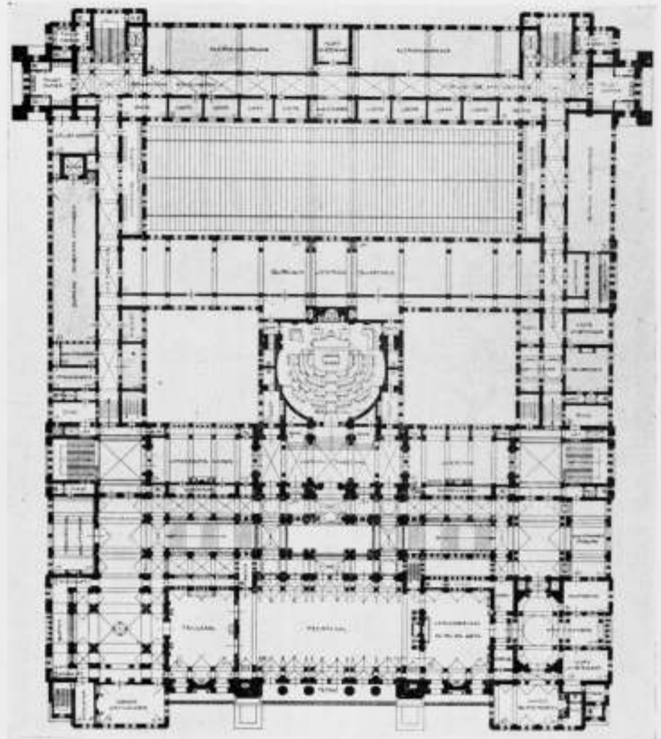
HOOFVERDIEPING.
