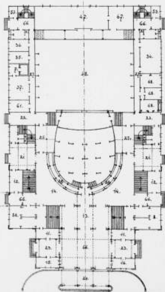
Begane grond:
