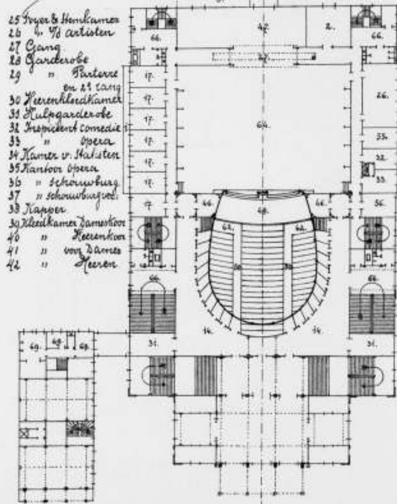
Parterre Verdieping:
